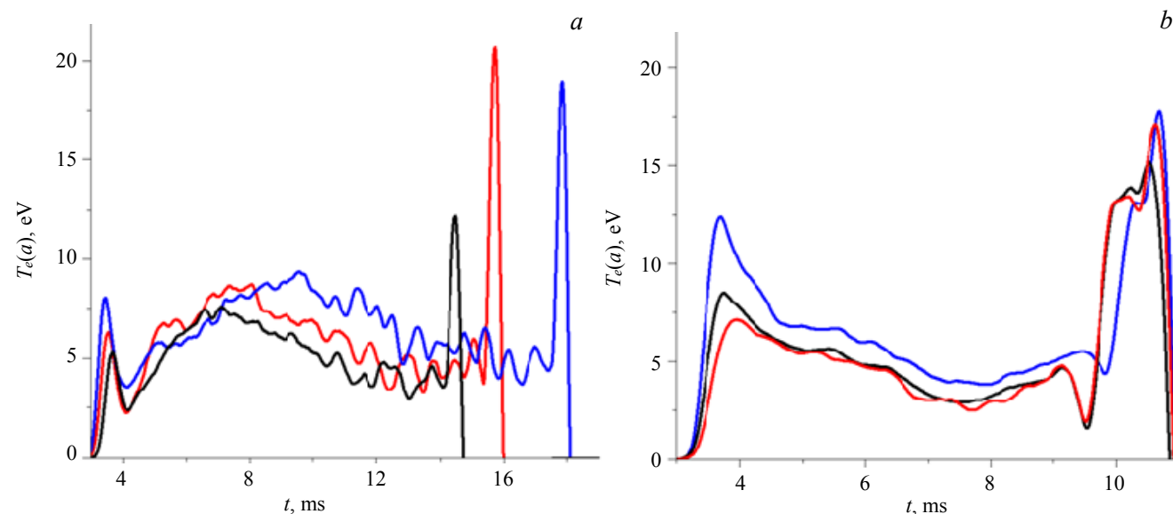
Fig. 14. Time evolution of the edge electron temperature for hydrogen: — № 33 067, p = 65 , — № 33 065, p = 56 , — № 33 075, p = 31 mPa, (a); helium plasmas: — № 33 023, p = 68 , — № 33 022, p = 55 , — № 33 020, p = 31 mPa (b), as measured by Langmuir probe for shots with U_{\text{CD}} = 500 V
