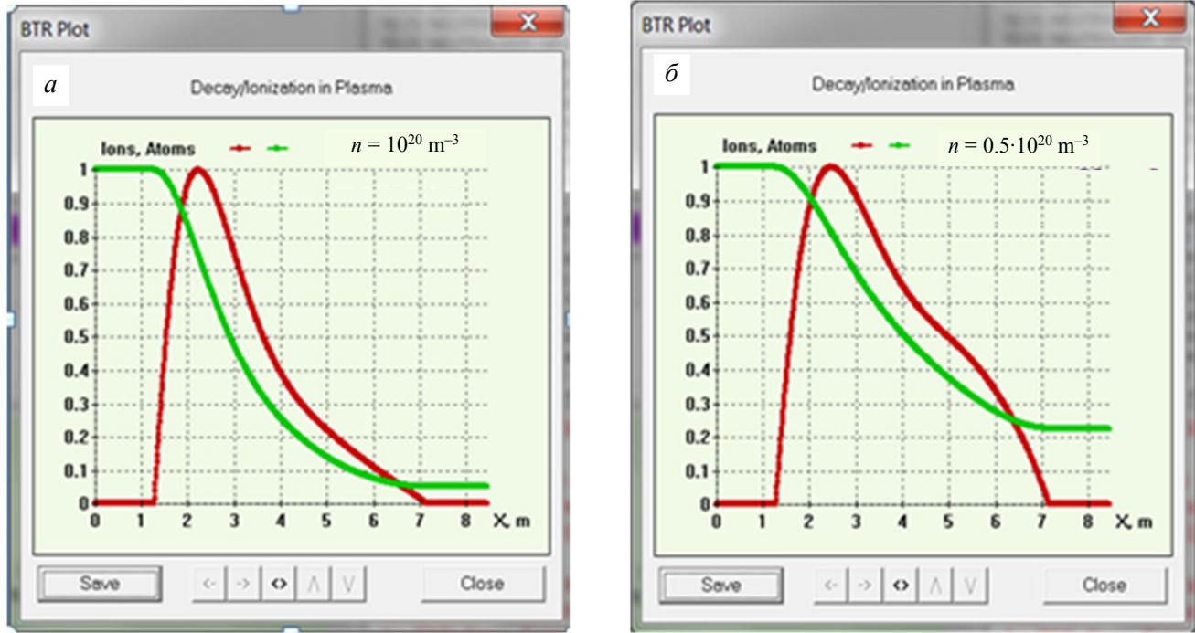
Fig. 4. BTR beam stopping in plasma: a , b — the beam species currents along beam axis (— atoms, — fast D + ) — for two values of plasma density
