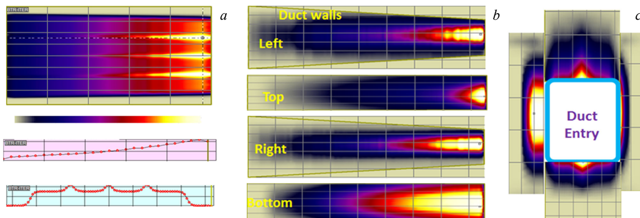
Fig. 8. BTR power maps and profiles used for thermal analysis: a — neutralizer wall; b — duct walls; c — scraper front
