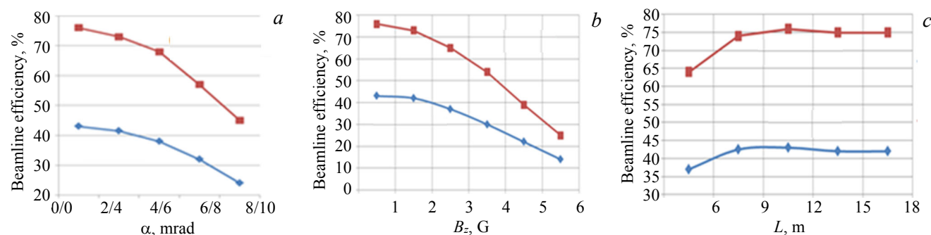
Fig. 7. Examples of NBI efficiency: NB misfocus effect (a), B_z effect at ideal focus (b), beamlet focusing distance (within a group) (c): geometry transmission ( P_{inj}/P_{Neutr} ) (—), total efficiency ( P_{inj}/P_0 ) (—)
