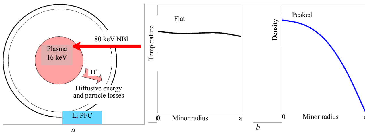
Fig. 2. (a) The LiWF regime with absorbing walls dramatically simplifies the physics. Energy goes to the wall with the core particle flux. (b) The temperature profile is flat, while the density profile is peaked
