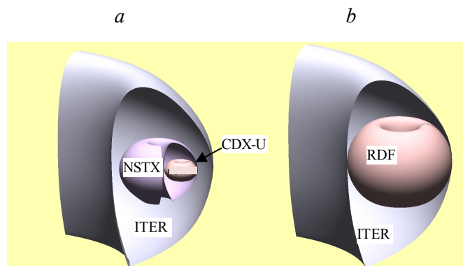
Fig. 7. Plasma configuration of (a) CDX-U and NSTX, experimental facilities for LiWF studies, and (b) the 0.2—0.5 GW Reactor Development Facility, considered as a feasible goal for the LiWF approach
