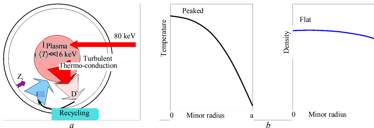
Fig. 1. (a) Conventional approach to magnetic fusion with the high recycling at the wall. (b) The temperature profile is peaked, while the density profile is flat
