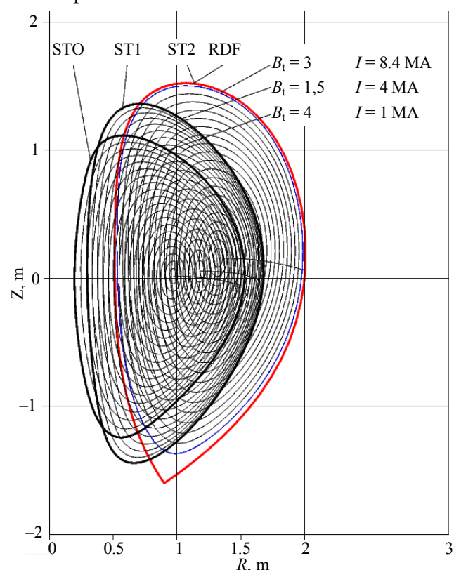
Fig. 6. Plasma cross-sections of NSTX (ST0), ST1, and identical ST2 and RDF
