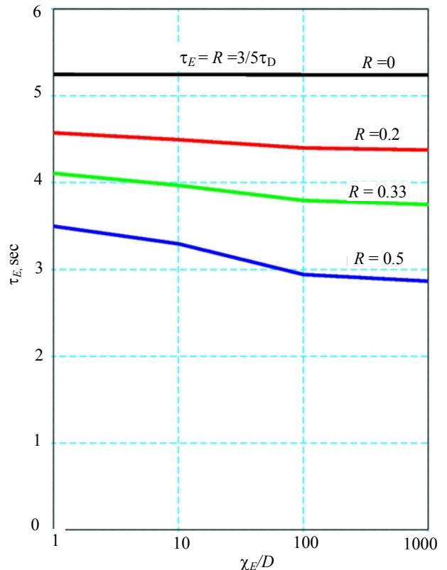
Fig. 5. Energy confinement time for ST1 device as a function of anomaly in the electron thermal conductivity for different recycling coefficients (gas injection is absent)
