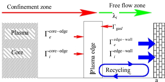
Fig. 4. Plasma edge, separating the core confinement zone and the "free" flow zone, and the plasma particle fluxes to the edge from the core side and from the wall side (including recycling and gas injection)
