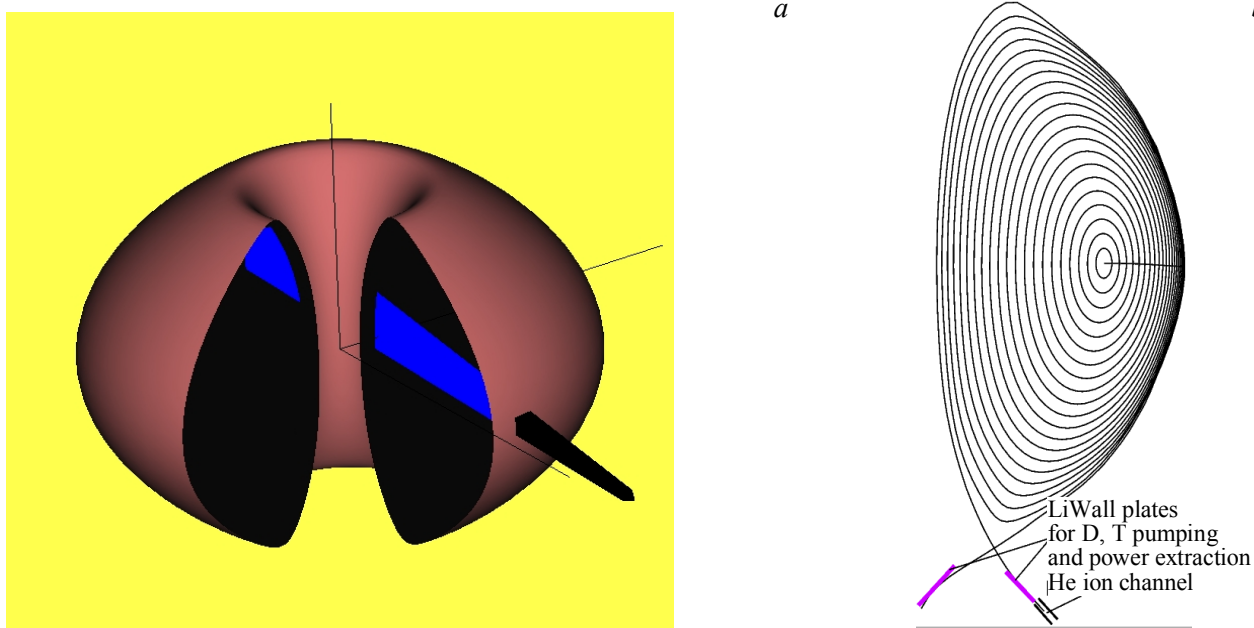
Fig. 3. Schematic implementation of LiWF in Spherical Tokamaks. (a) NBI fueling and heating the plasma.(b) Positioning the liquid lithium target plates in the divertor area for plasma particle pumping
